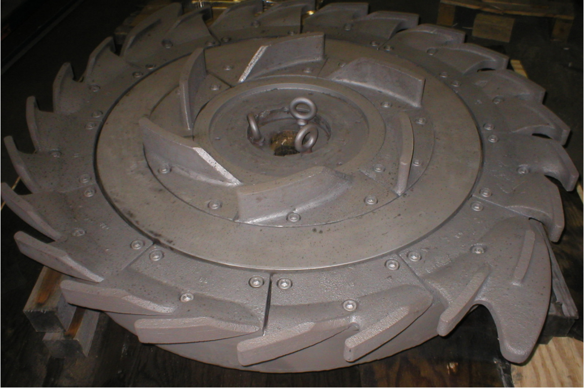
Rebuilt 60" Conventional Rotor
