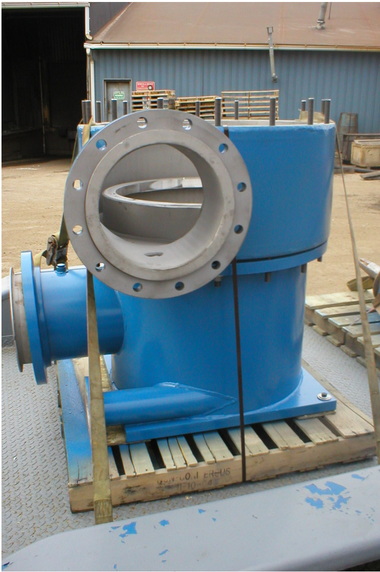
Rebuilt 24P Black Clawson Selectifier Screen Body
