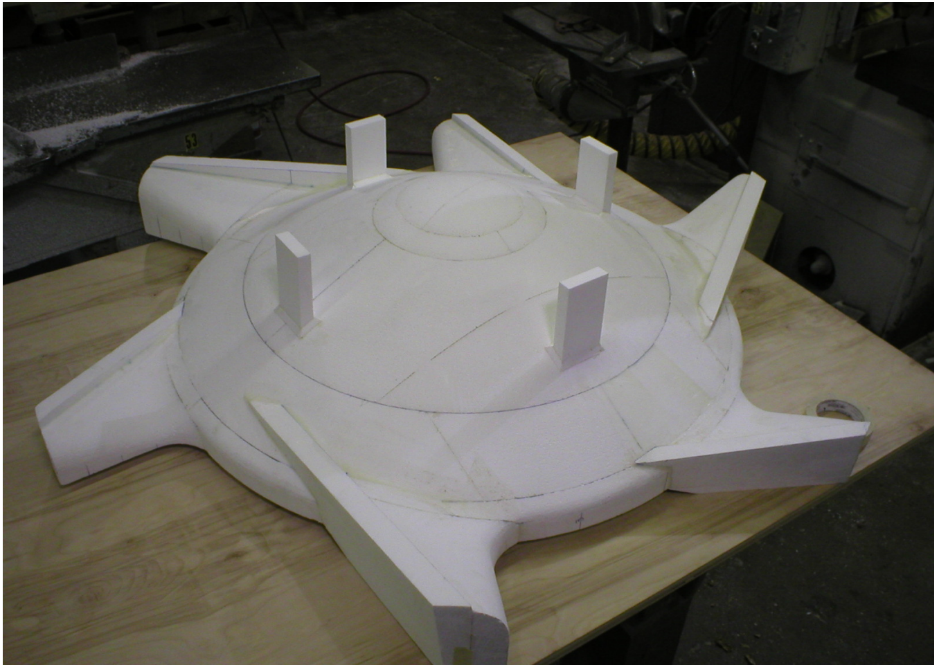
Disposable foam pattern for 55" Beloit Shark rotor
